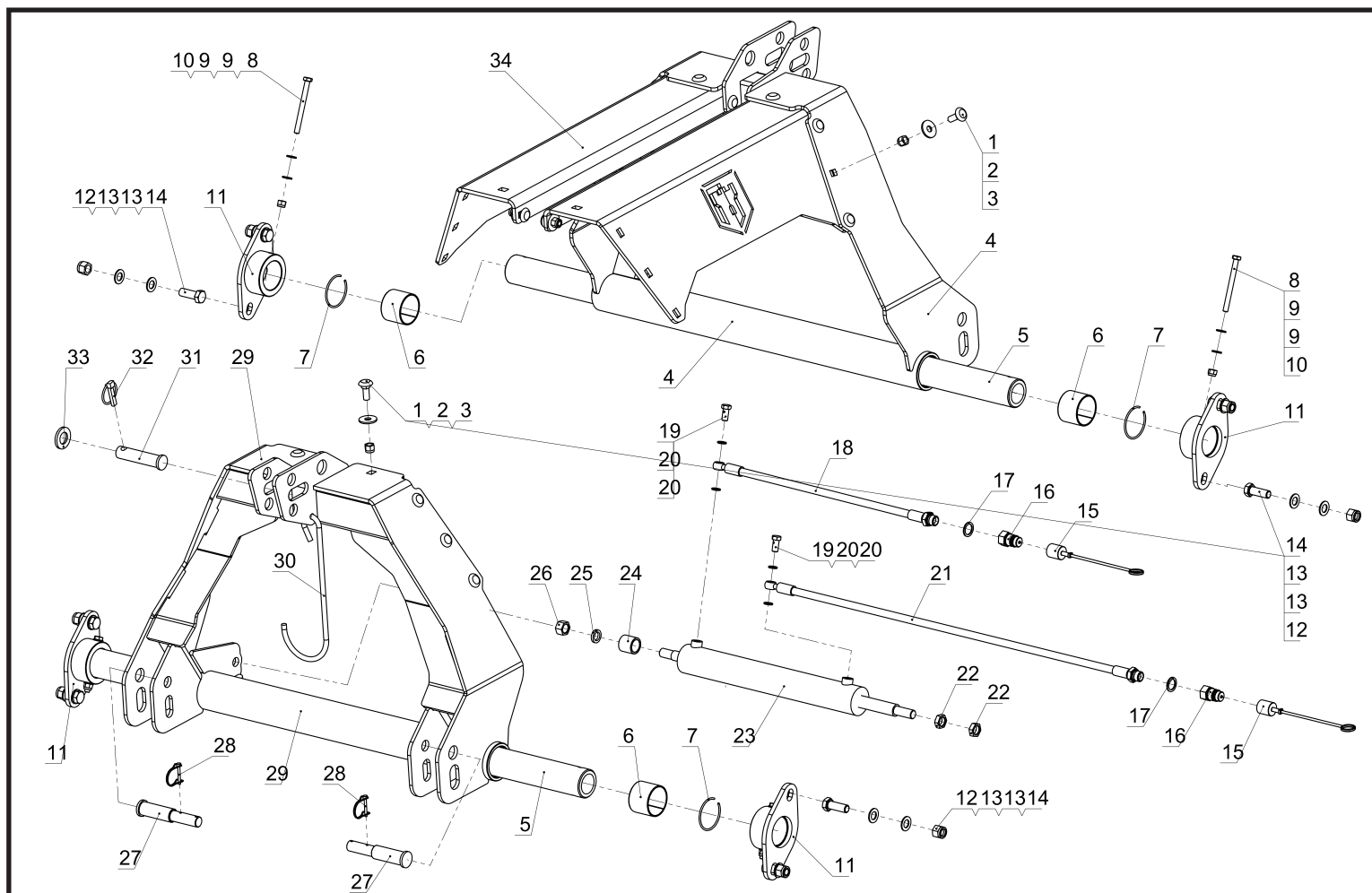
SHARK PROFI three-point linkage
